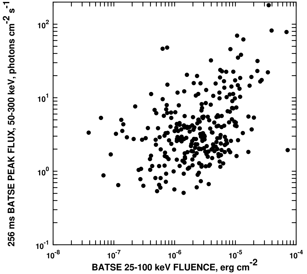
Fig. 9.— Peak fluxes (measured over 256 ms, 50-300 keV) and 25-100 keV fluences of 272 of the bursts in this catalog. No entries are given in the 5B catalog for 71 of the bursts.
