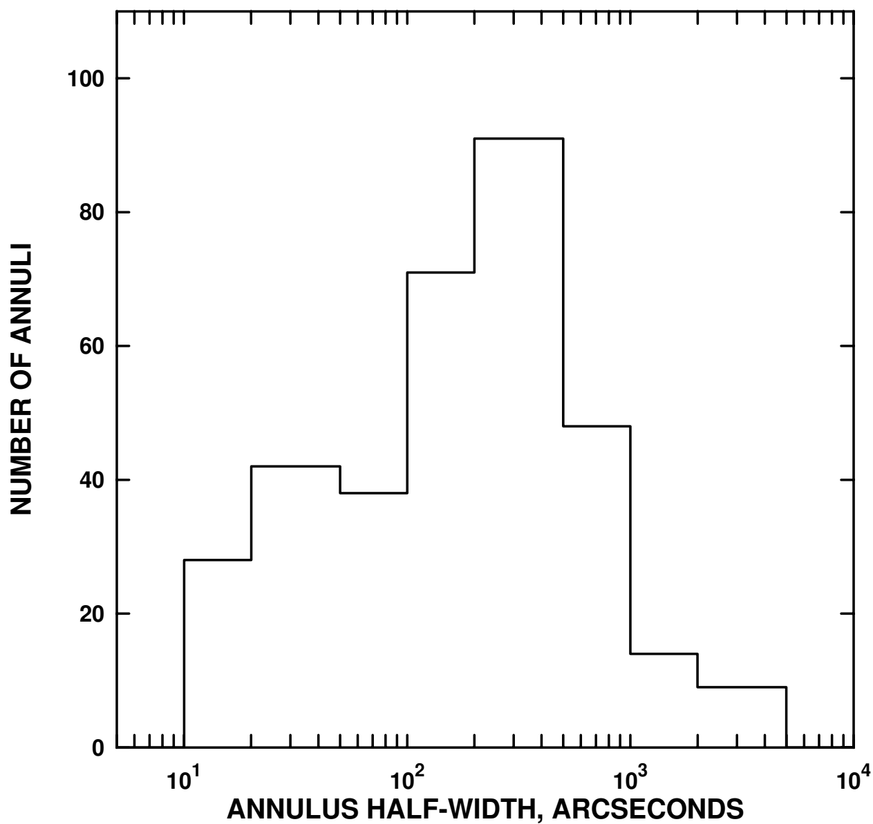
Fig. 7.— Distribution of 343 IPN annulus half-widths.
