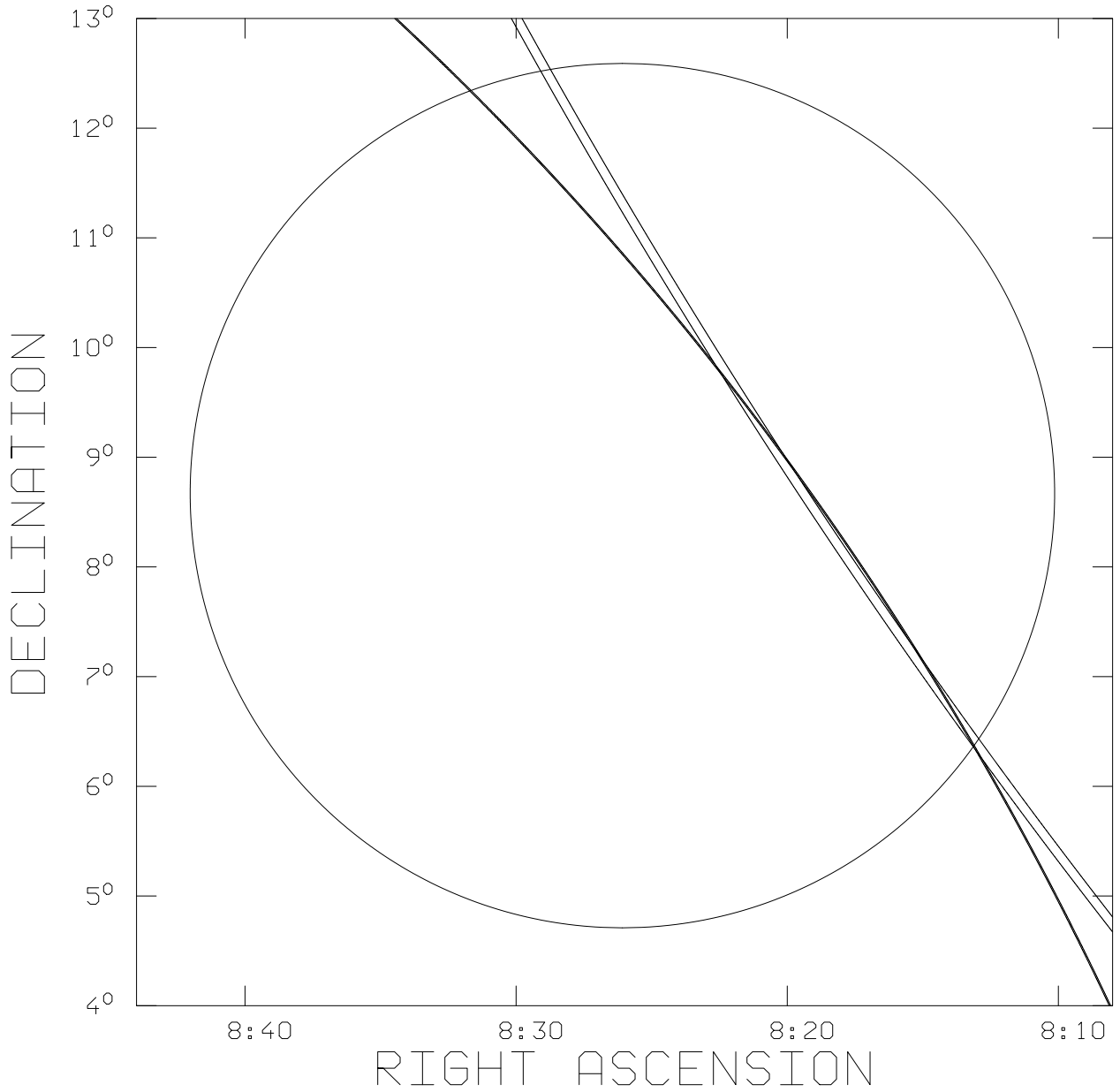
Fig. 6.— The BATSE 1\sigma (statistical + systematic) error circle for trigger 7647 on 1999 July 12, and the 3\sigma Ulysses -BATSE and NEAR - BATSE annuli. the two annuli intersect nearly at grazing incidence, defining two error boxes within the BATSE error circle.
