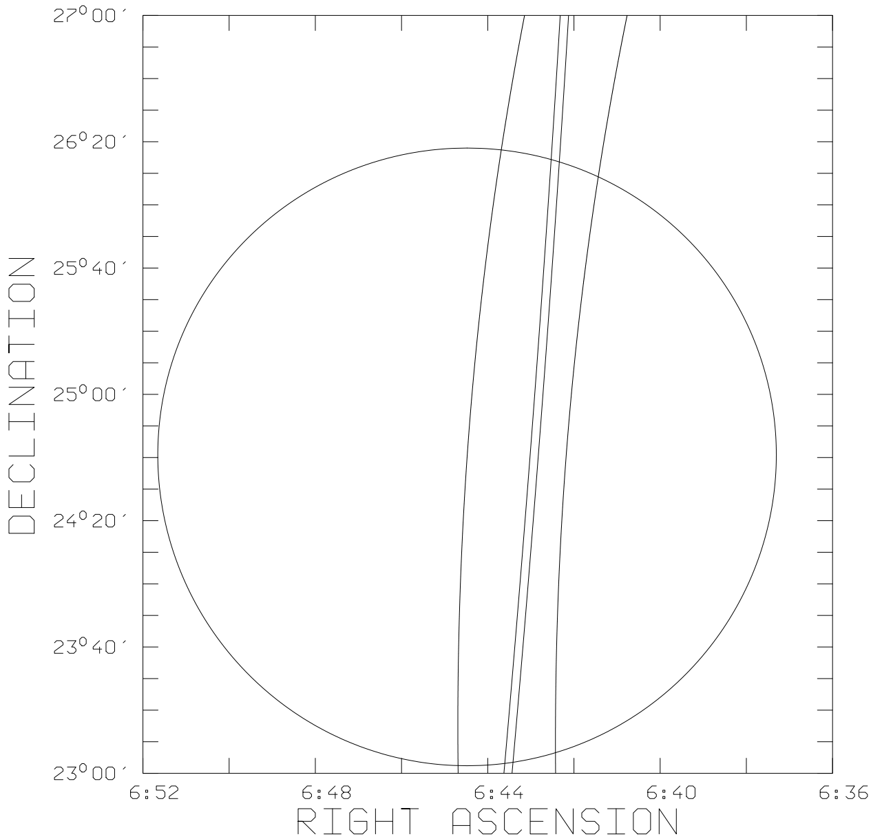
Fig. 5.— The BATSE 1\sigma (statistical + systematic) error circle for trigger 6453 on 1997 October 29, and the 3\sigma Ulysses -BATSE and NEAR - BATSE annuli. Again, the NEAR-BATSE annulus is wider. Because the two annuli intersect at grazing incidence, they define a single error box whose length is much greater than the radius of the BATSE error circle.
