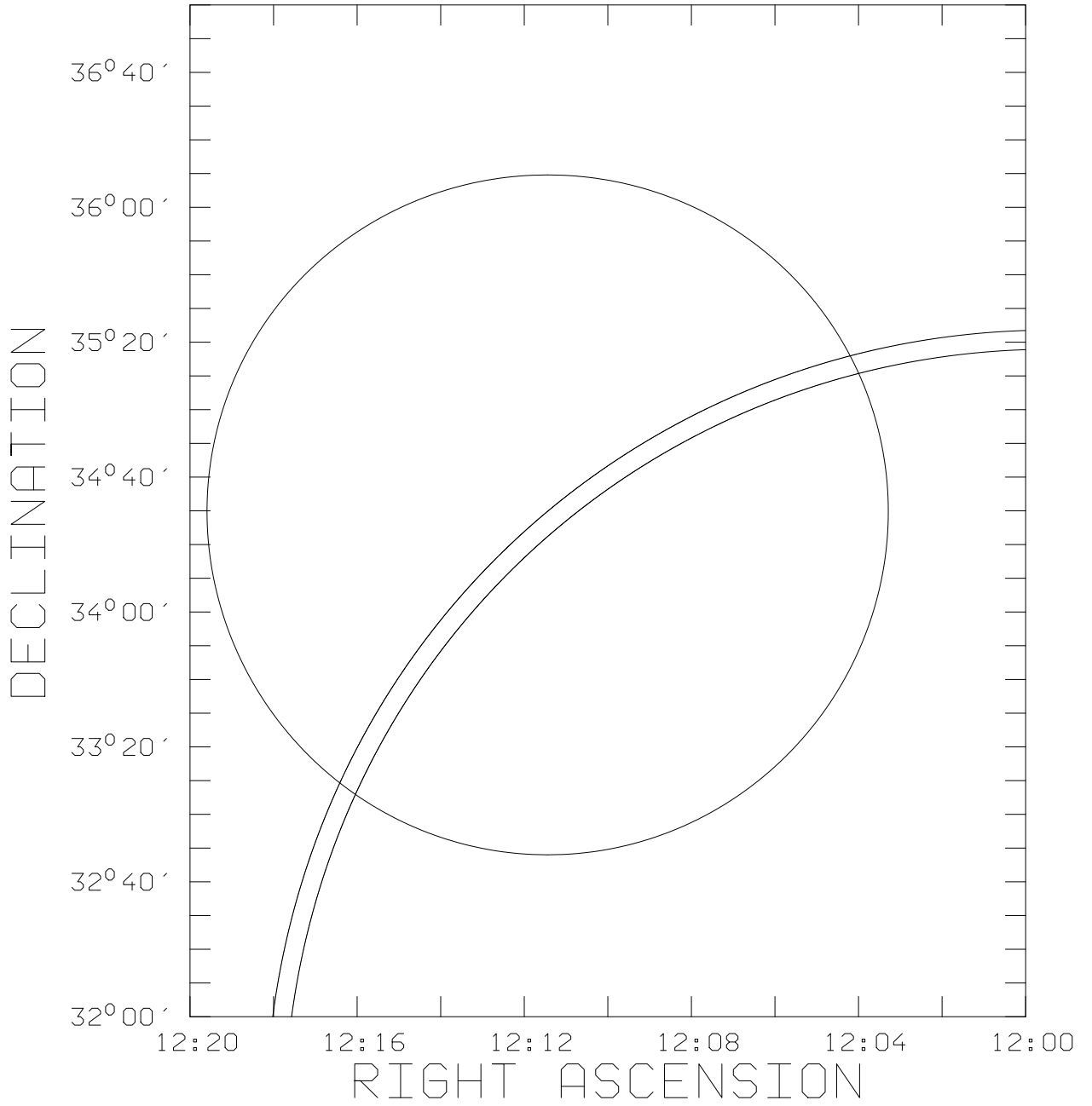
Fig. 3.— The BATSE 1\sigma (statistical + systematic) error circle for trigger 5711 on 1996 December 12, and the 3\sigma IPN annulus. The curvature of the annulus makes it impossible to describe the resulting error box with the four annulus/error circle intersection points.
