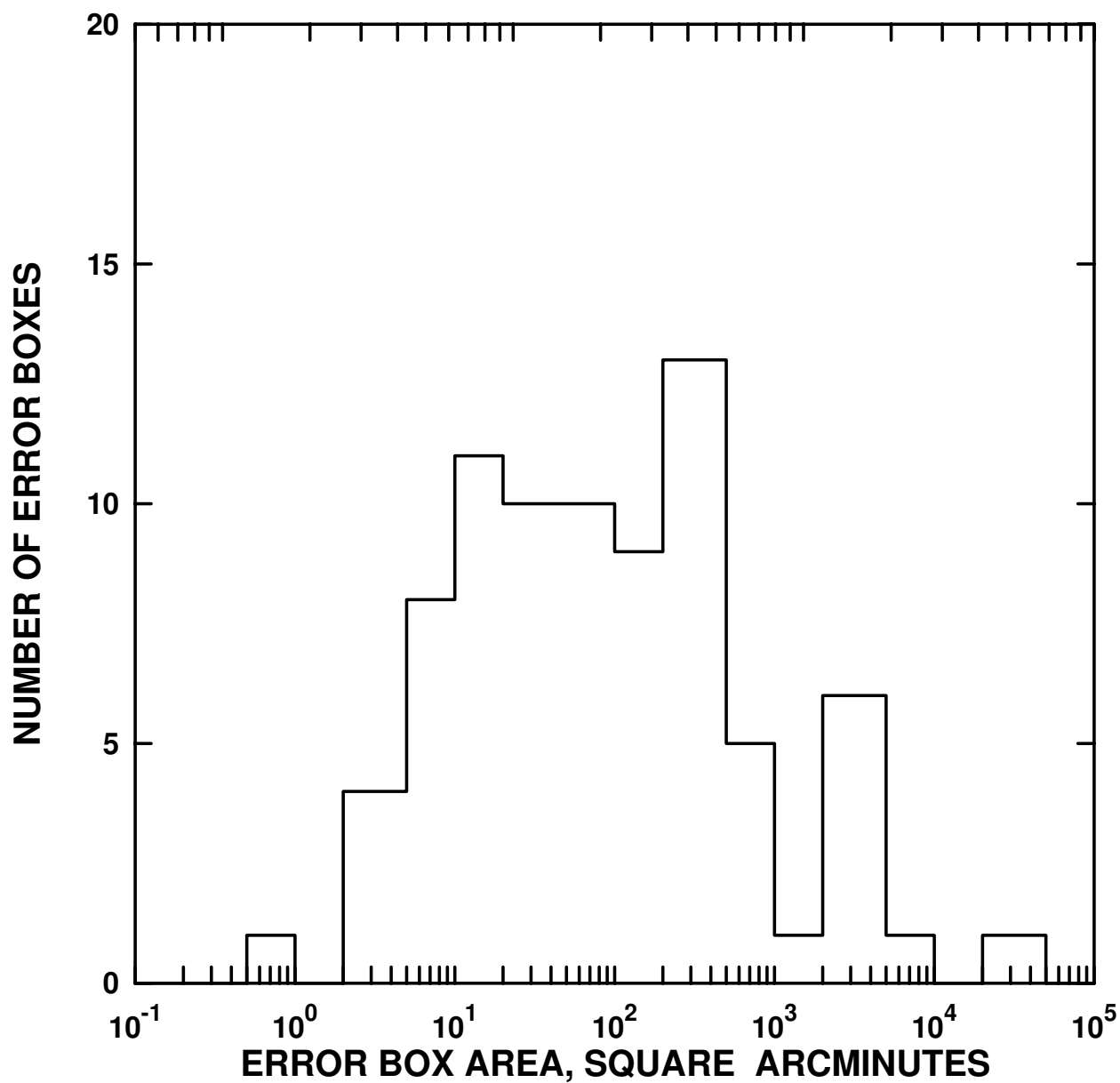
Fig. 8.— Distribution of 80 IPN error box areas.
