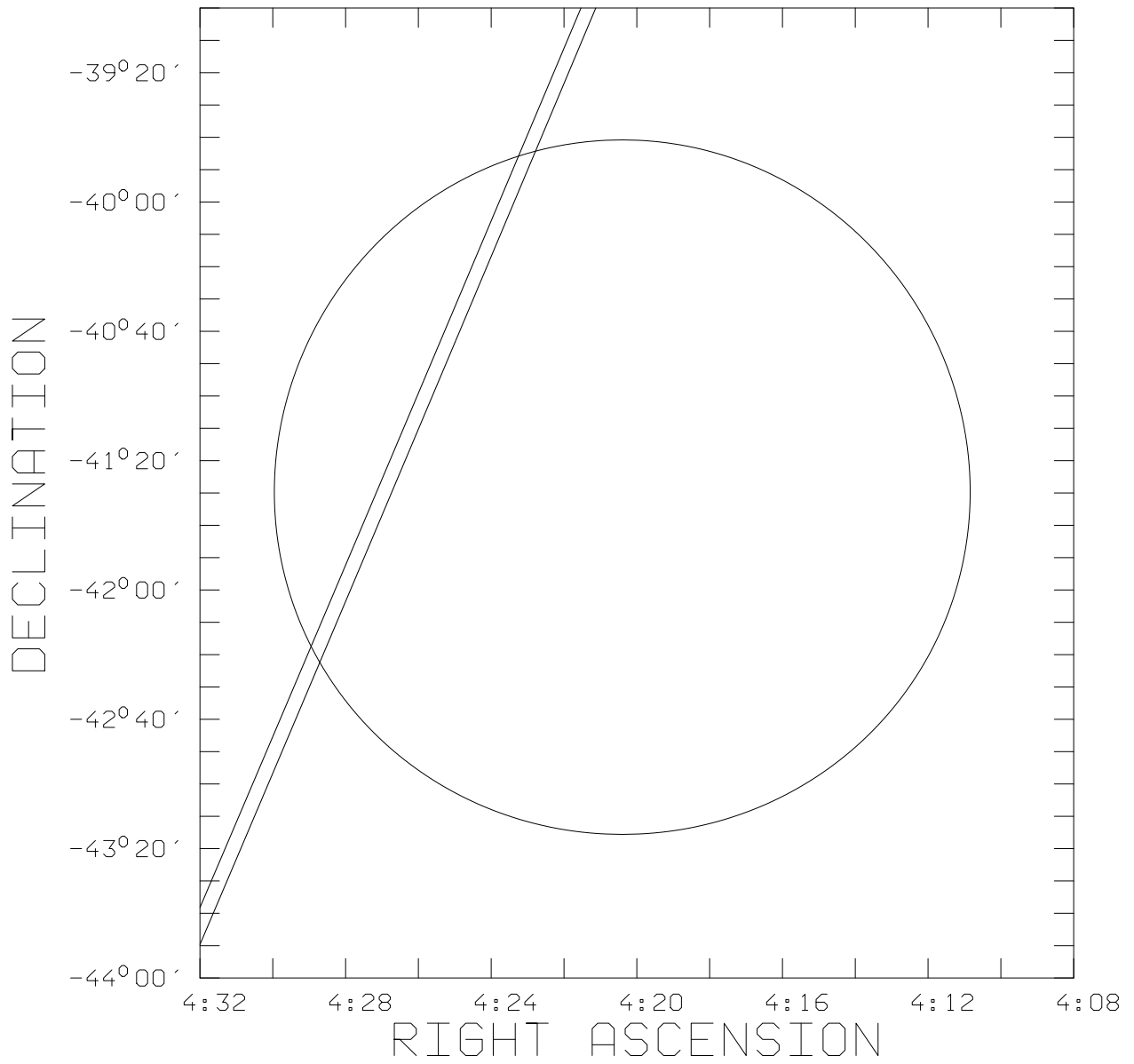
Fig. 2.— The BATSE 1\sigma (statistical + systematic) error circle for trigger 5593 on 1996 September 6, and the 3\sigma IPN annulus.
