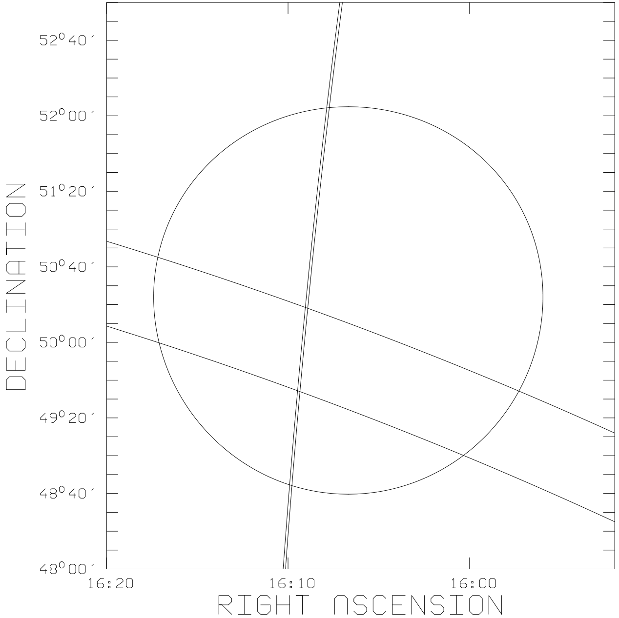
Fig. 4.— The BATSE 1\sigma (statistical + systematic) error circle for trigger 6472 on 1997 November 10, and the 3\sigma Ulysses -BATSE and NEAR - BATSE annuli. Because NEAR was closer to Earth than Ulysses (smaller D in equation 2), and had only 1 s time resolution (resulting in a larger \sigma(\delta T) in equation 2), the NEAR-BATSE annulus is wider.
