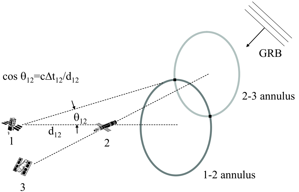
Fig. 1.— The triangulation technique. Each independent spacecraft pair is used to derive an annulus of location for the burst. Three spacecraft produce two possible error boxes. The ambiguity can be eliminated by the addition of a fourth, non-coplanar spacecraft, or by the anisotropic response of one of the detectors.
